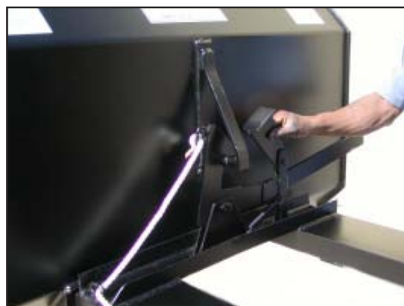
Safety Lock prevents accidental tripping of bucket during transportation.
