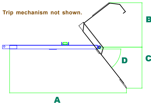
Illustration shows bucket in dump position.
